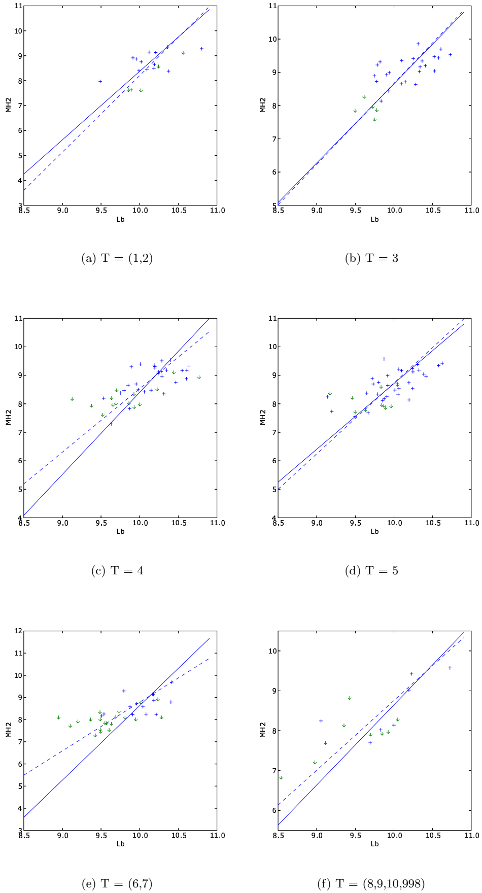
Figure 9.13: M_{H_2} - L_B as a function of morphology. Dashed line represents the fit to the detected galaxies and the full line corresponds to the fit using survival analysis.
